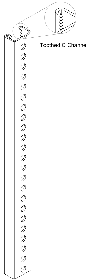
ISOMETRIC VIEW
