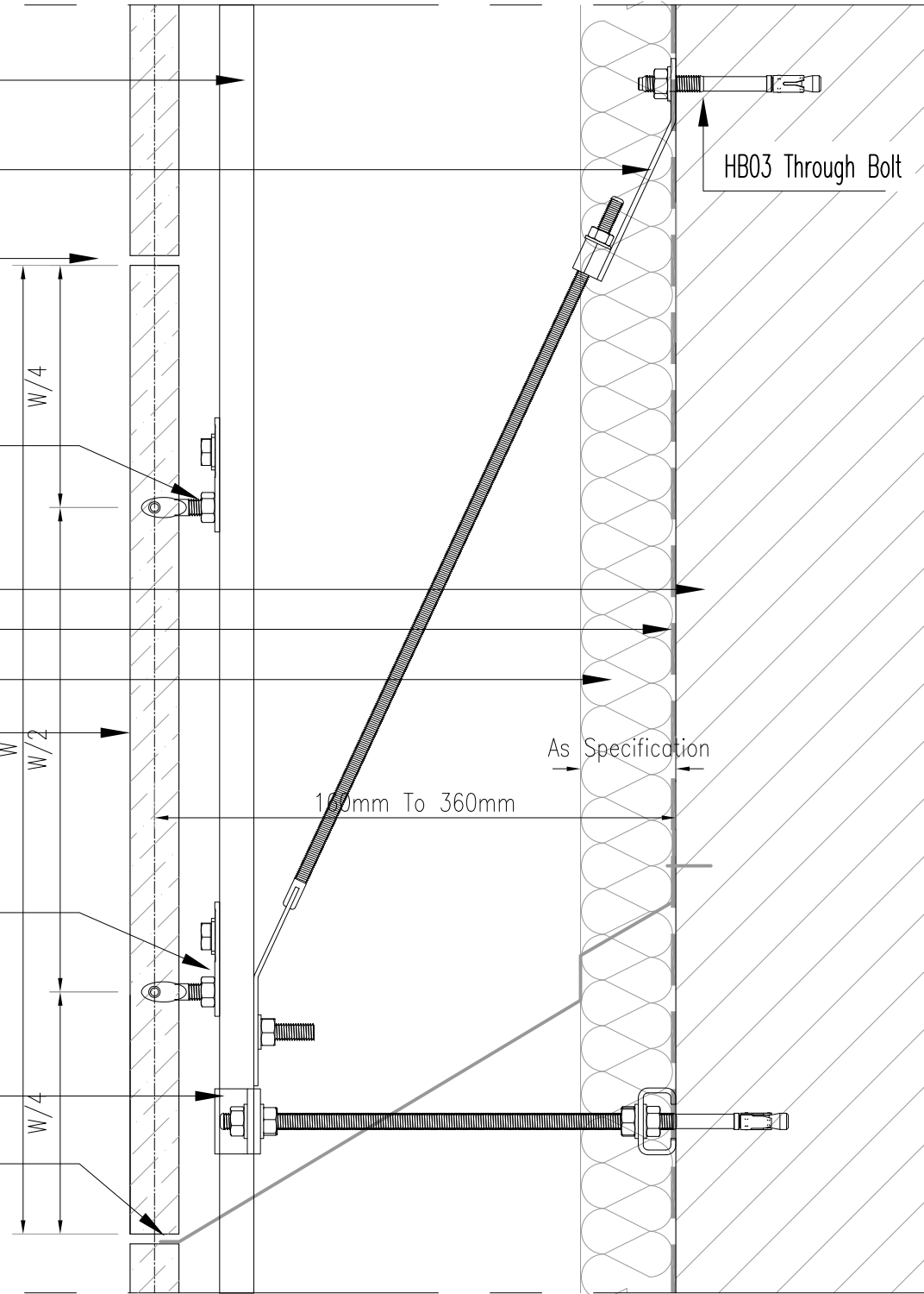
Vertical section Scale 1:4
