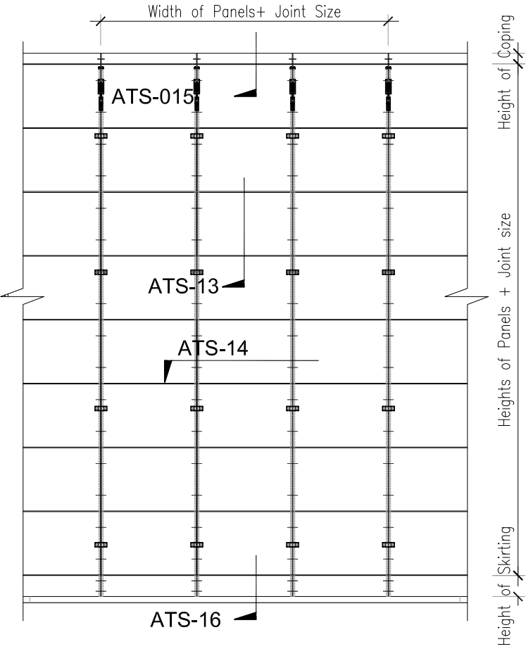
Elevation Scale 1:50
