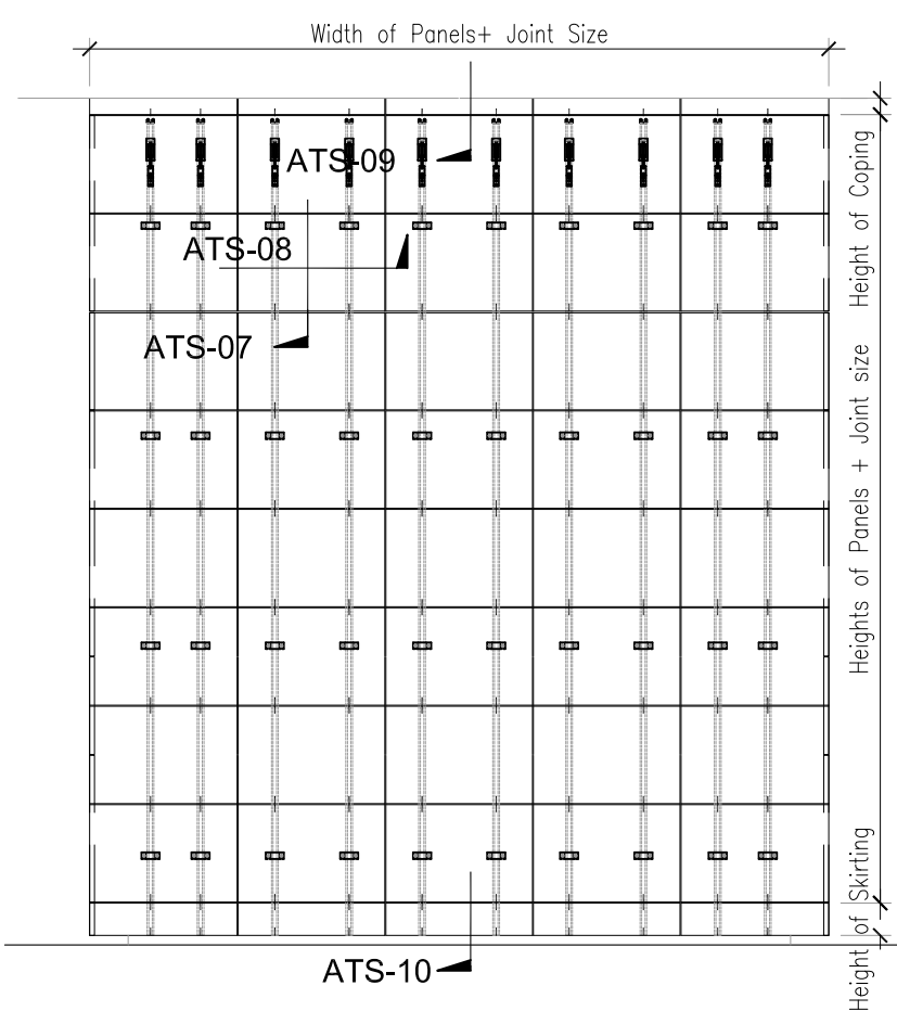
Elevation Scale 1:50
