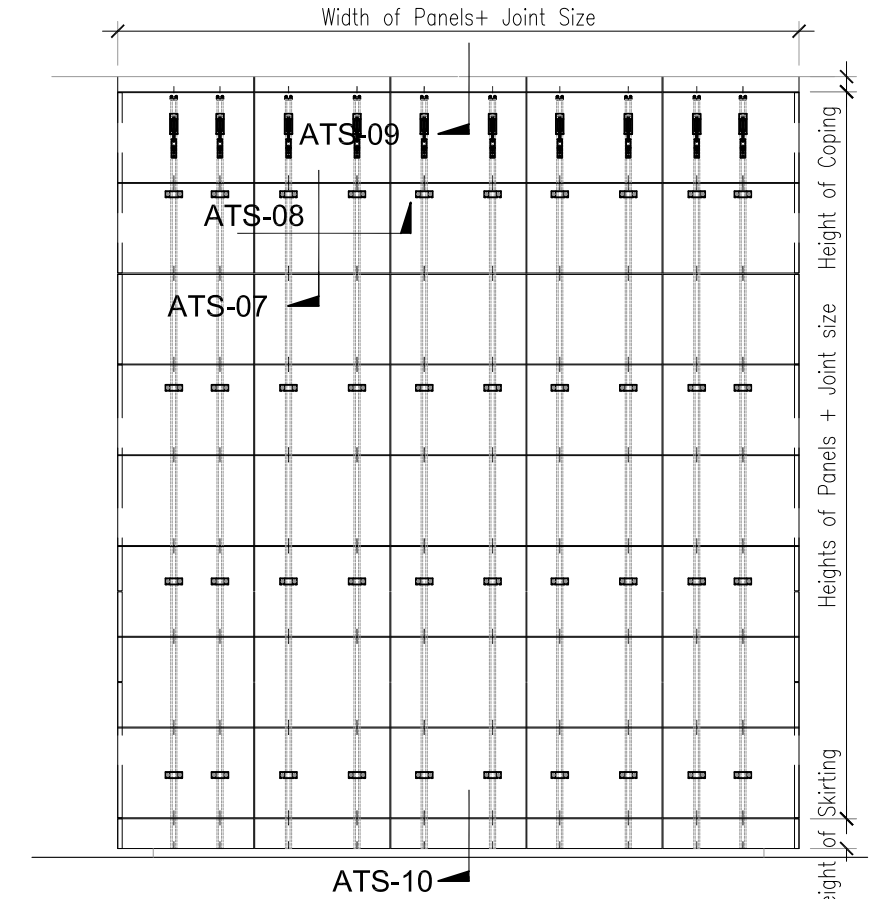
Elevation Scale 1:50
