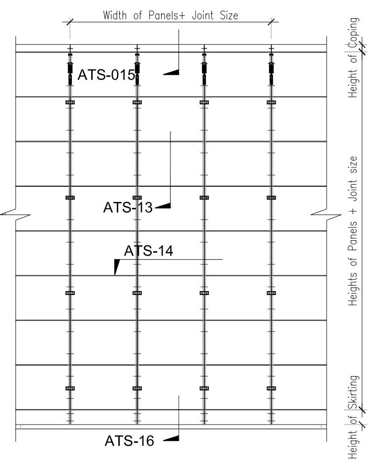
Elevation Scale 1:50
